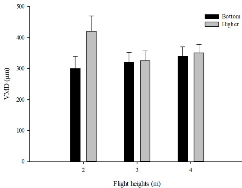
Figure 5: Effect of the operational application height and the canopy layer of conilon coffee on VMD.
