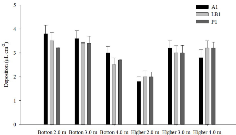
Figure 6: Effect of operational height and height range of the plant on deposition.
