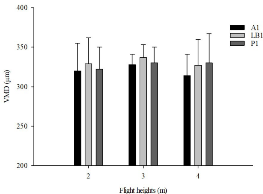
Figure 4: Effects of flight heights and genotype and their interactions for the variables VMD.
